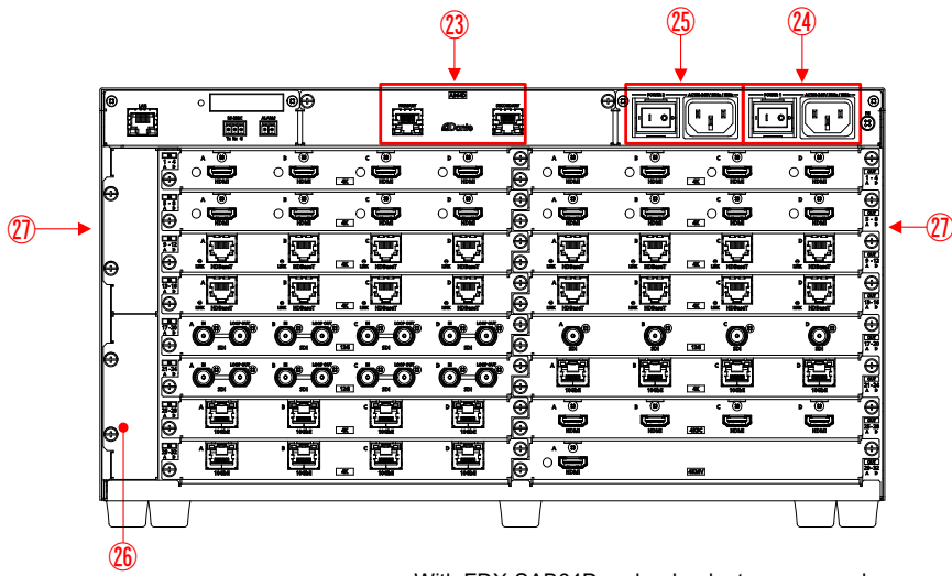
[Fig. 5.3] Drawings
