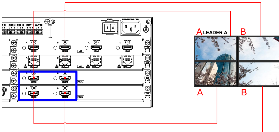
[Fig. 10.12] Synchronization (2×2 videowall by two output boards with 4K@60 scan converter)
