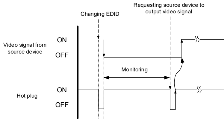
[Fig. 10.18] Monitoring absence of input
