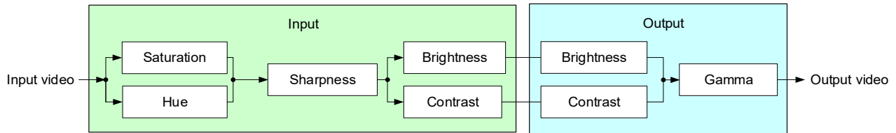
[Fig. 10.22] Picture controls
