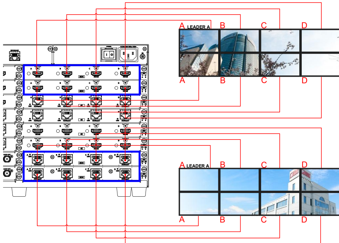
[Fig. 10.10] Synchronization (Example: Two 4×2 videowall)
