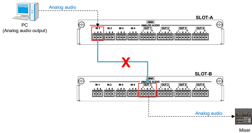
[Fig. 8.9] Audio cannot be transmitted between an audio boards between installed audio boards
