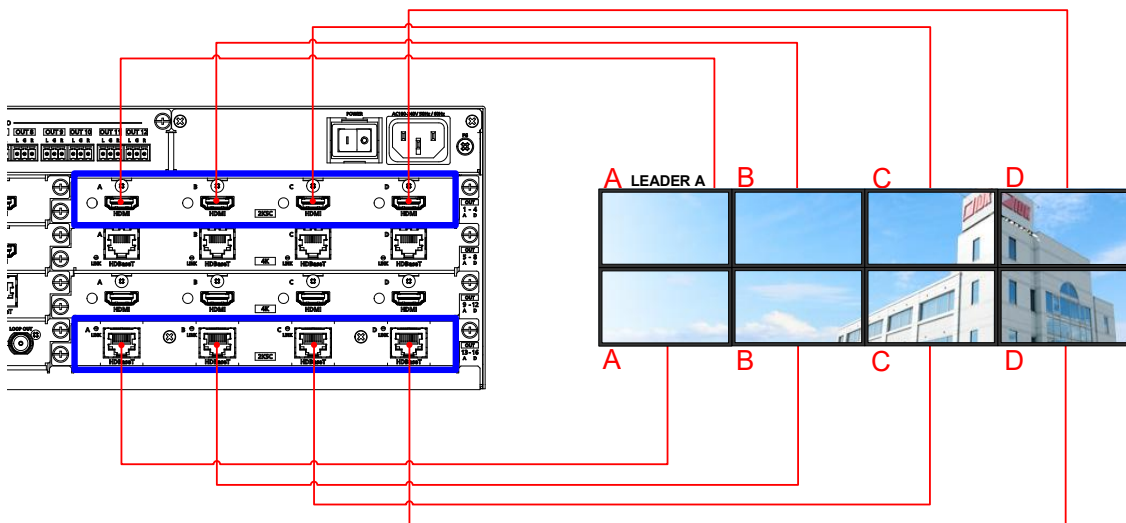
[Fig. 10.11] Synchronization setting (4×2)
