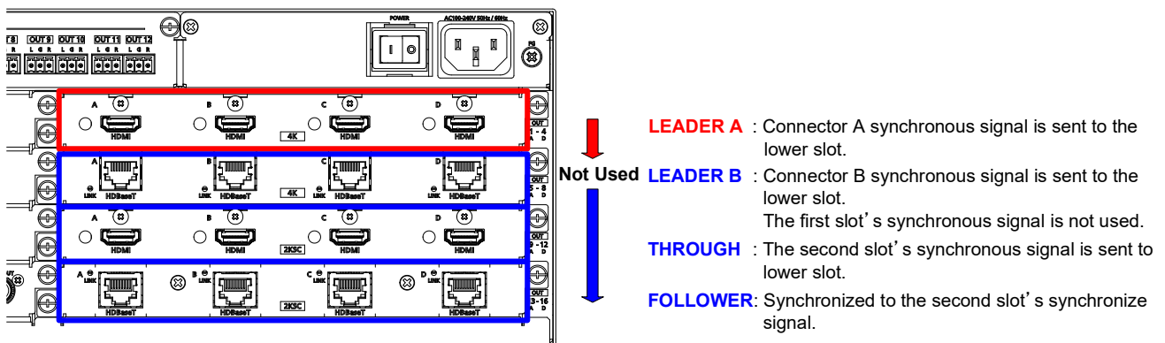
[Fig. 10.8] Sending synchronous signal
