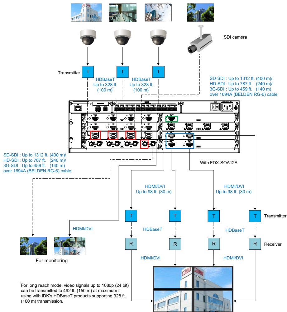
[Fig. 8.1] Connecting video devices (Example: FDX-S08U)
