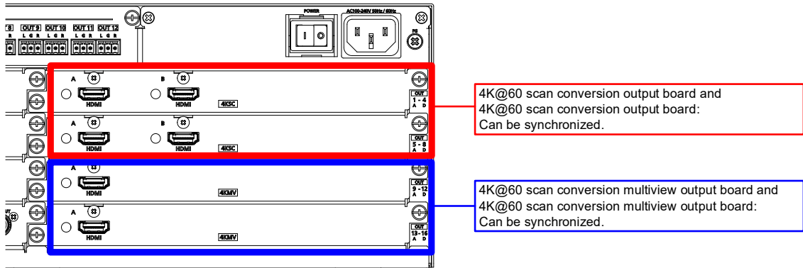
[Fig. 10.15] Example (Can be synchronized)
