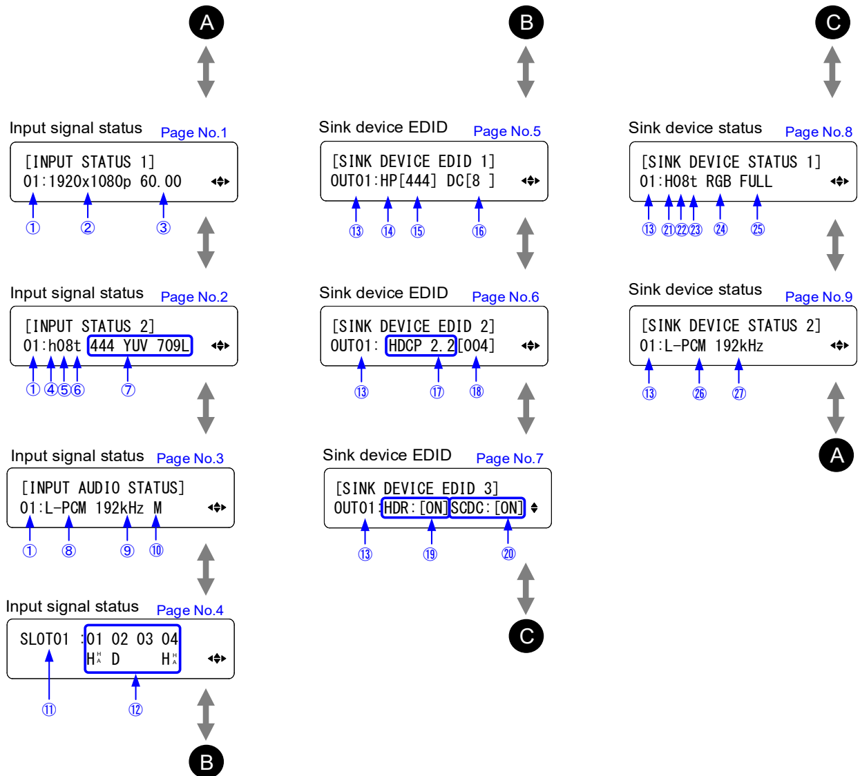
[Fig. 10.49] Top page of front display
