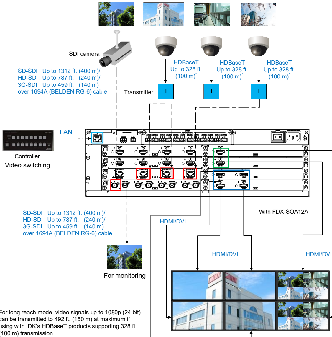
[Fig. 6.1] System configuration example (Example: FDX-S16U)
