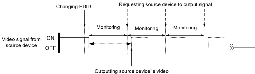
[Fig. 10.19] Repeating output reset
