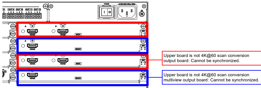
[Fig. 10.16] Example (Cannot be synchronized)
