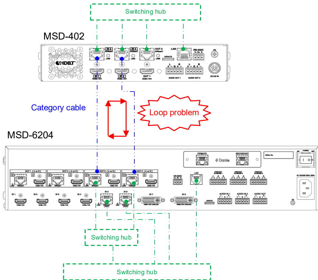
[Fig. 9.25] Loop problem with IDK's device (Example: MSD-6204 with Dante)
