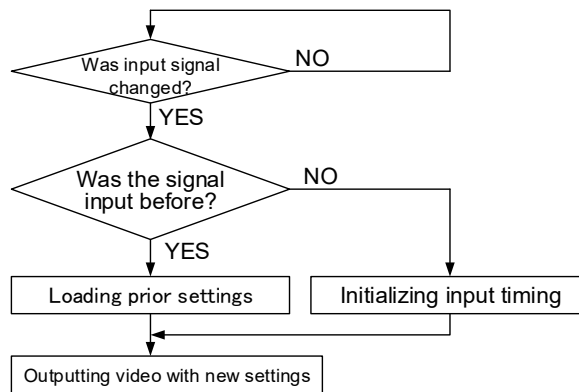
[Fig. 9.4] How input signals are recognized
