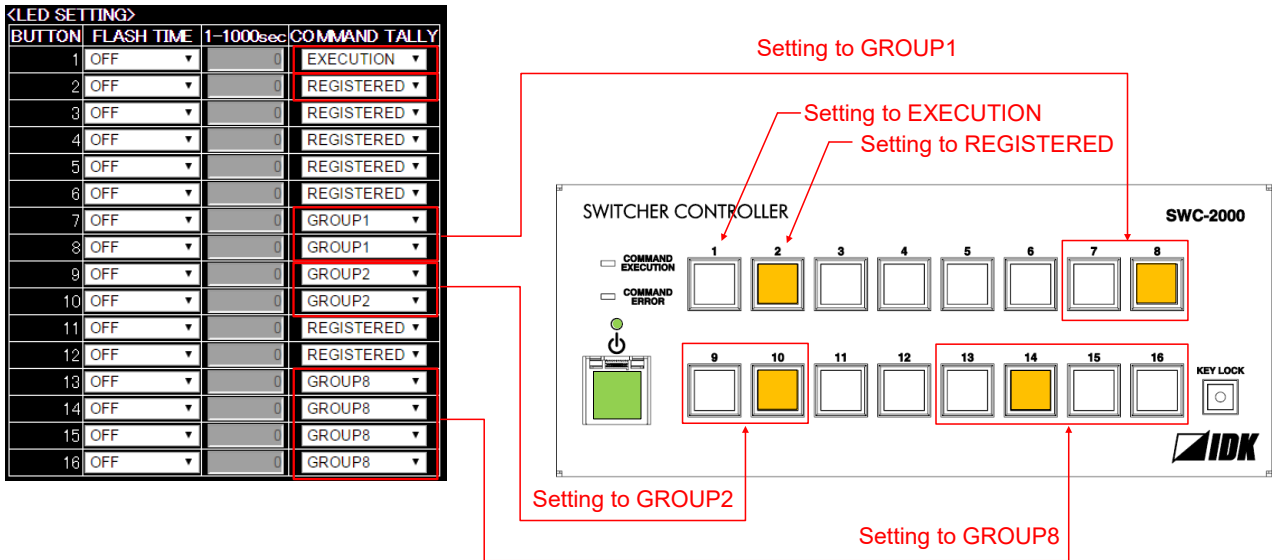
[Fig. 9.37] Grouping control command buttons
