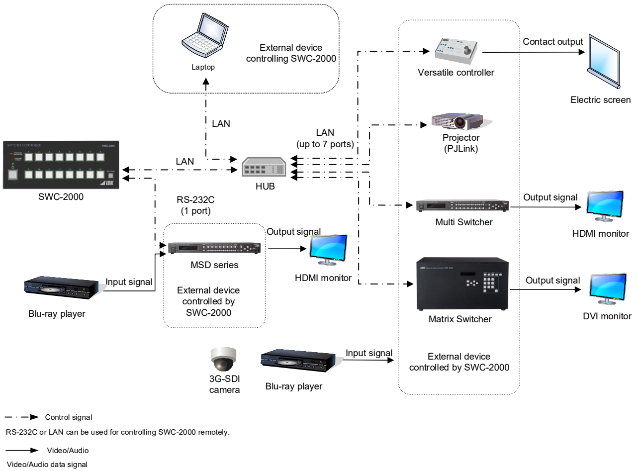
[Fig. 6.3] System application example
