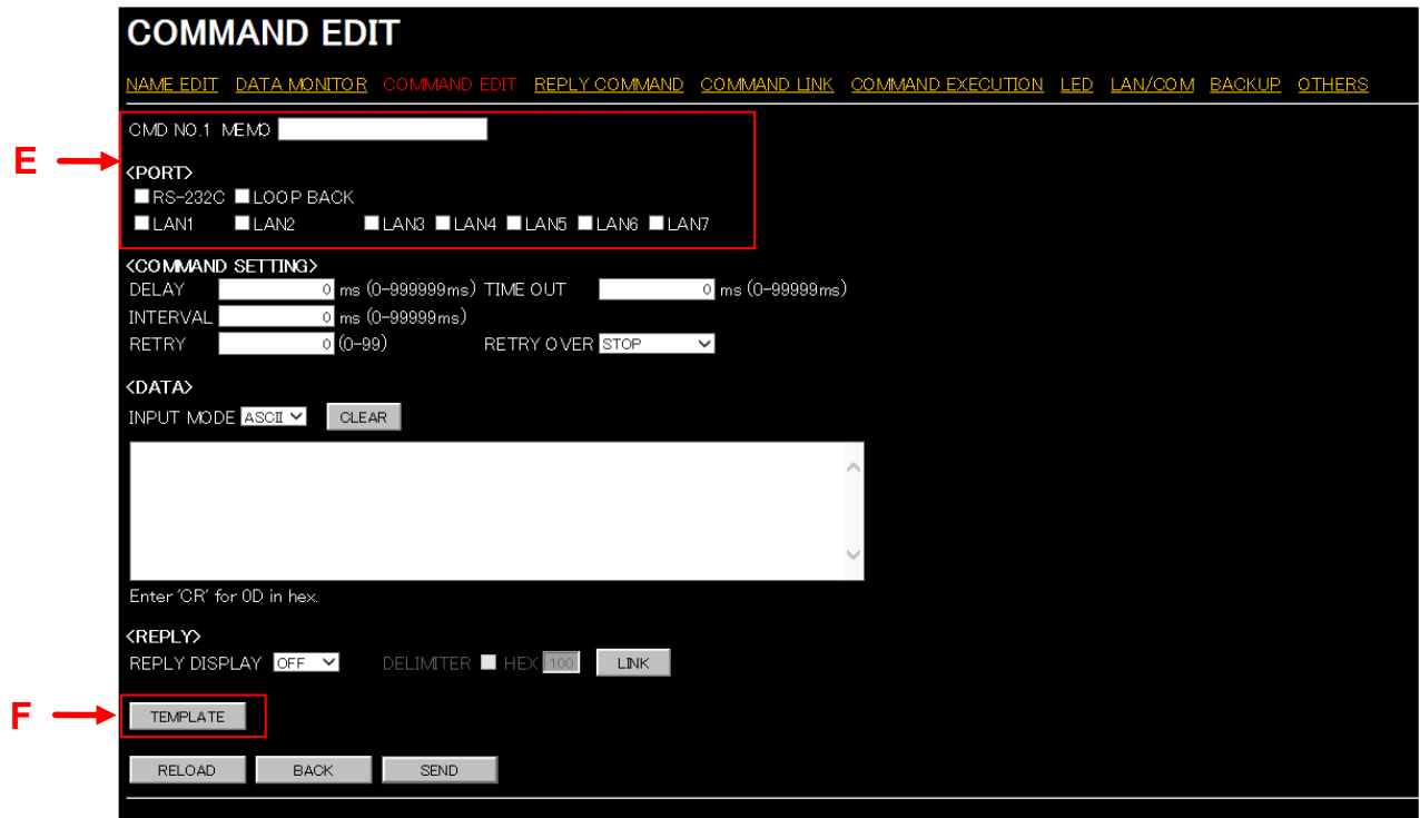
[Fig. 8.4] Advanced setting page for control command
