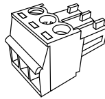
3-pin captive screw connector VAC-S12U × 2 VAC-S14U × 1 VAC-S16U × 1 VAC-S18U × 1
