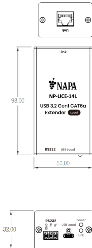
NP-UCE-14L (Local Unit)
