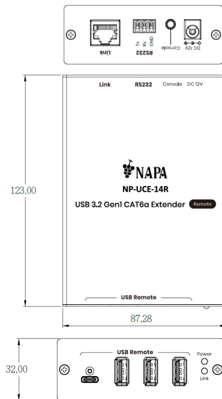
NP-UCE-14R (Remote Unit)
